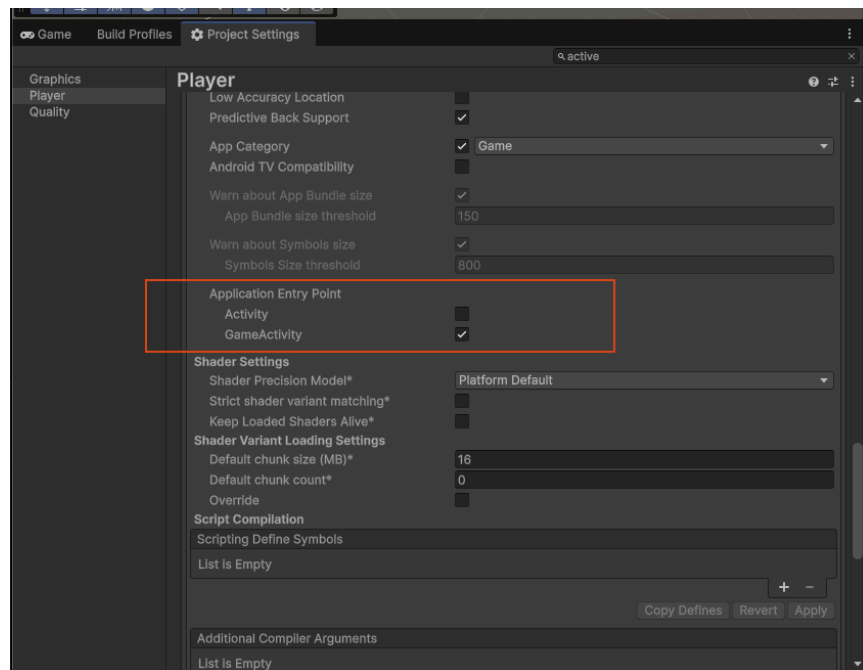
Player settings — make sure Game Activity is the entry point.
